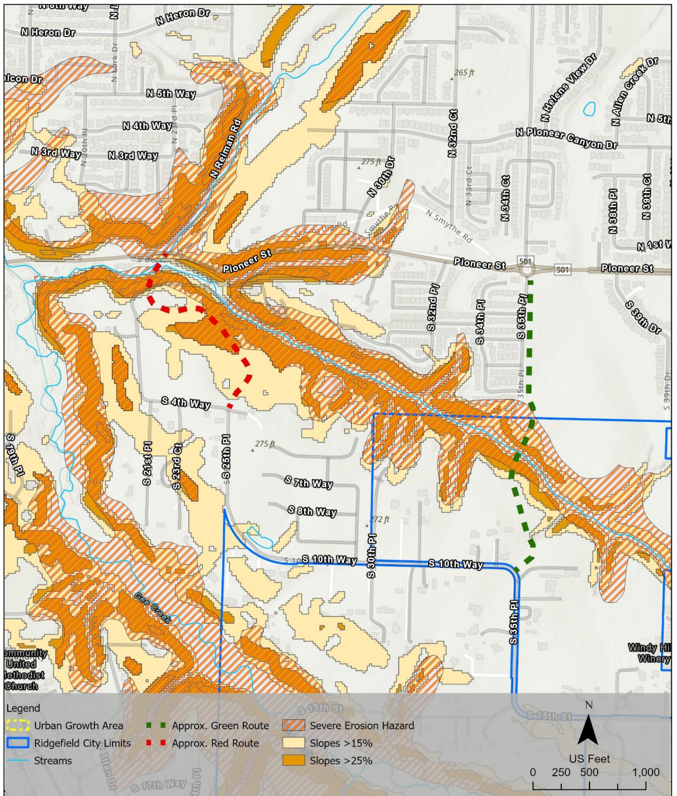
Figure 10. Steep Slopes
