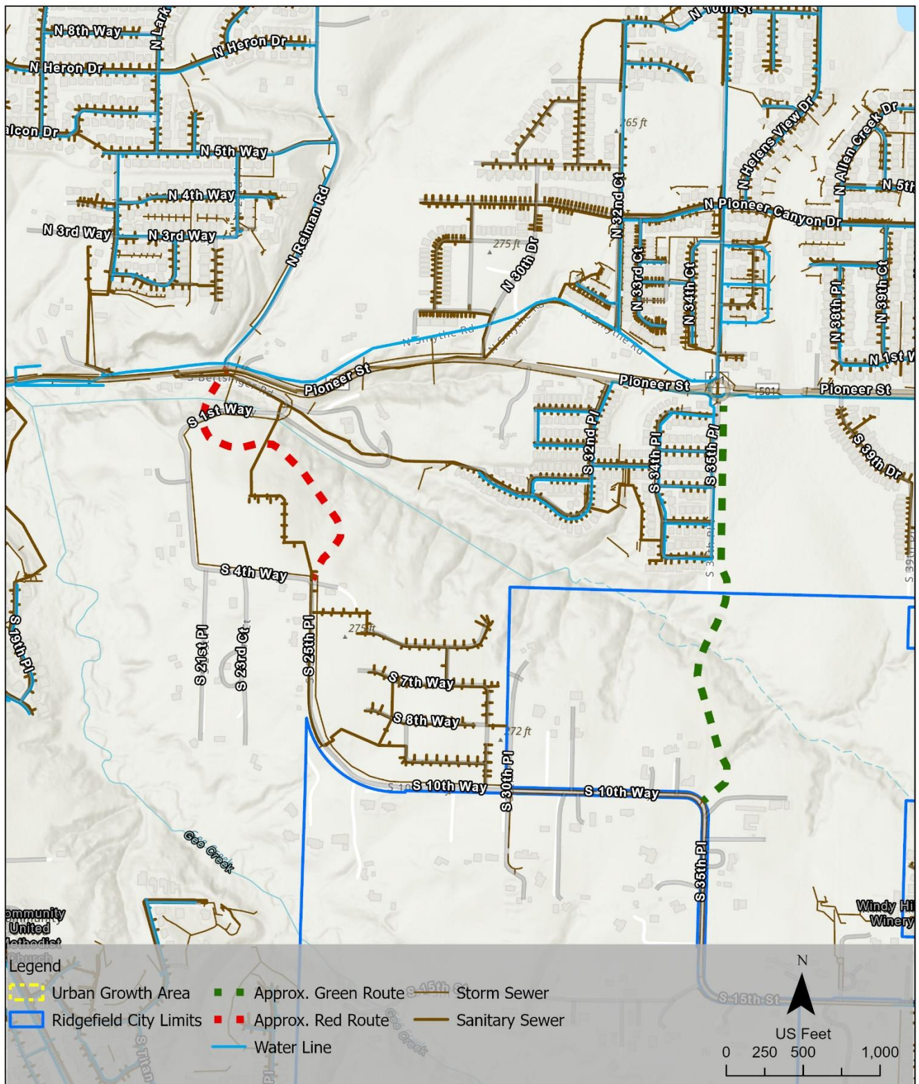
Figure 11. Existing Utilities
